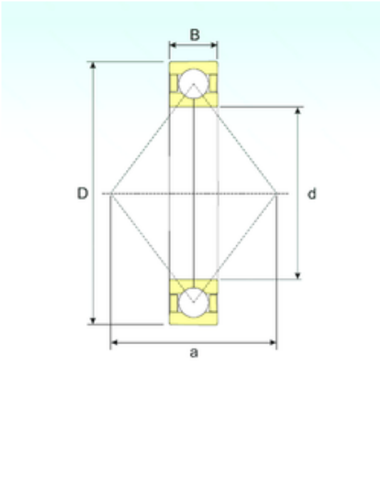
QJ 306 N2 M Bearing 2D drawings and 3D CAD models
